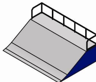
S1122 Bank 150-29-625
